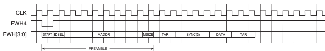
Figure 6-1. FWH Single-byte Read Waveforms
